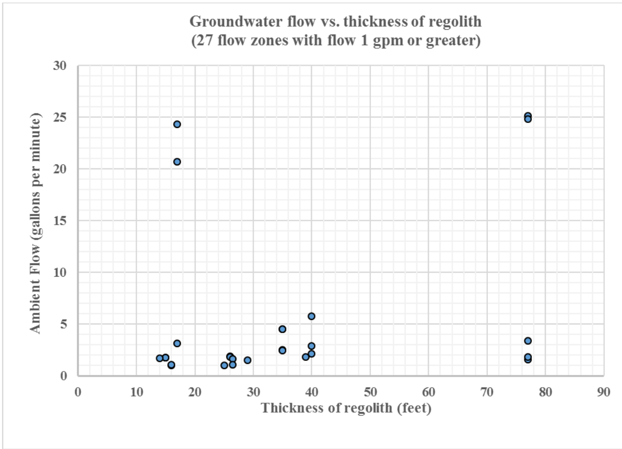
Figure 5.—Relationship of magnitude of groundwater flow (ambient) to thickness of regolith for 27 largest flows of 436 flow zones in RSA wells.
